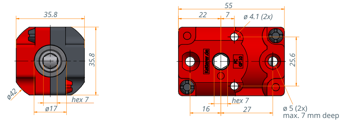
3045.00-3001 - Ratio 1:1
